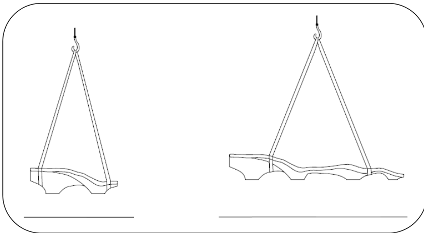
Fig. 1 – Crane install – strap locations
