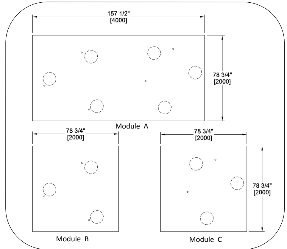
Fig. 2 – Plan views
